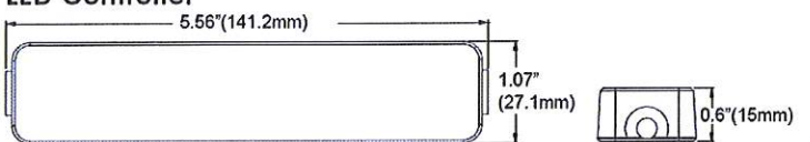
LED Controller
